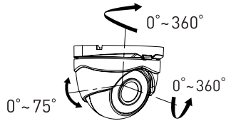
Figure 2-4 3-axis Adjustment
