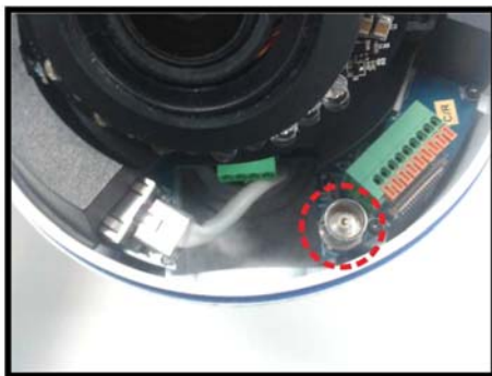
Built-In BNC Connector
