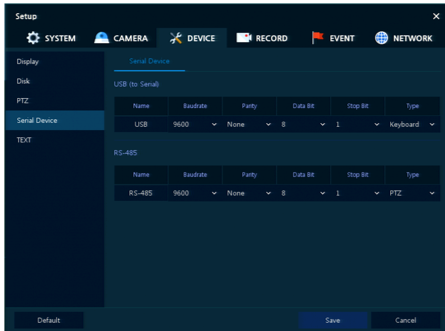
Figure 4-24 DEVICE > Serial Device > Serial Device
