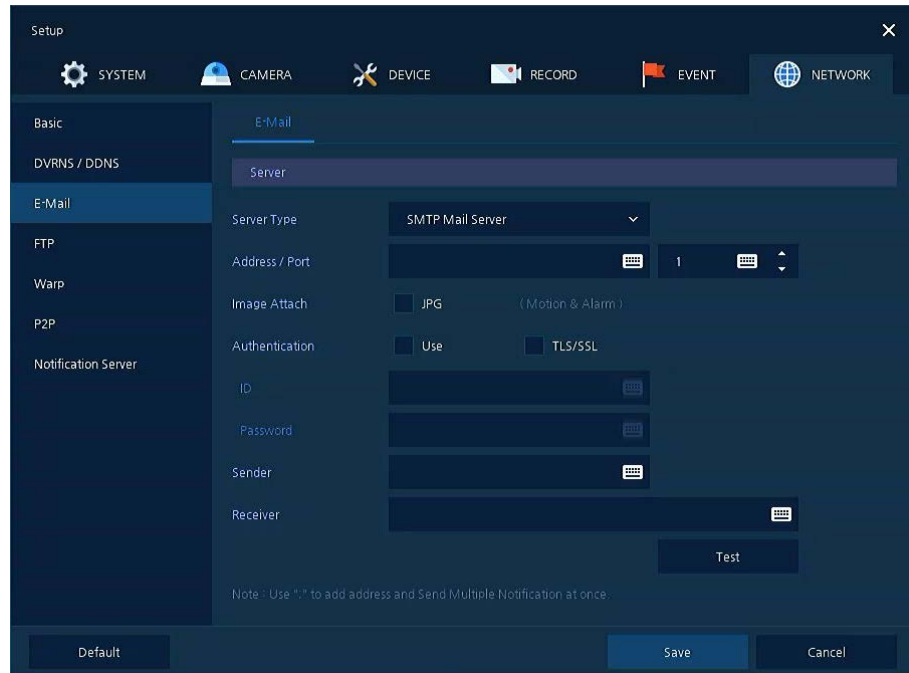
Figure 4-46 NETWORK > E-Mail > E-Mail
