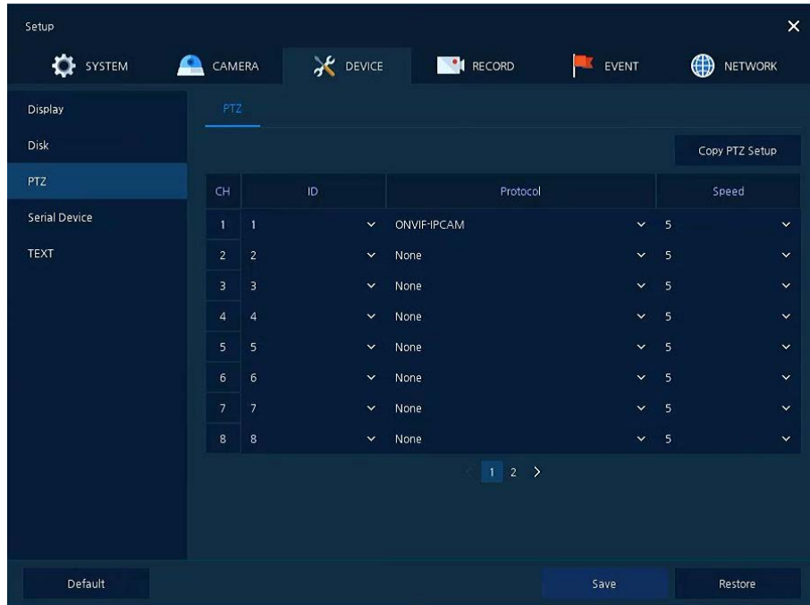
Figure 4-23 DEVICES > PTZ > PTZ
